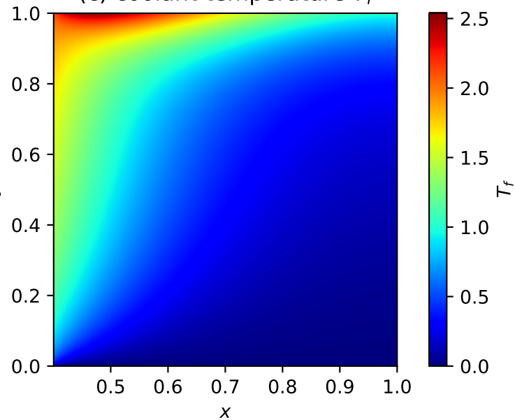
(c) coolant temperature T_f
