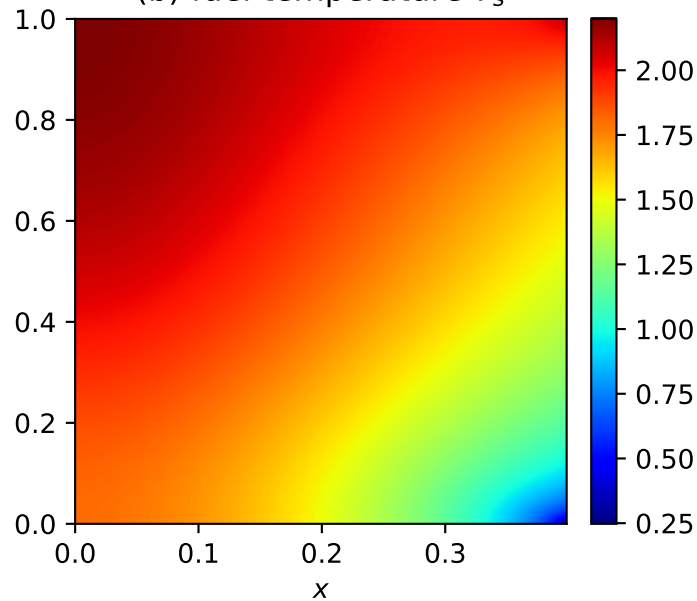
(b) fuel temperature T_s
